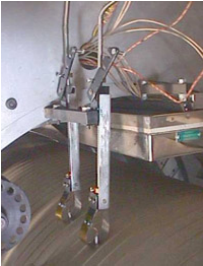
Thermocouple assy. for continuous rotating surface measurement.
